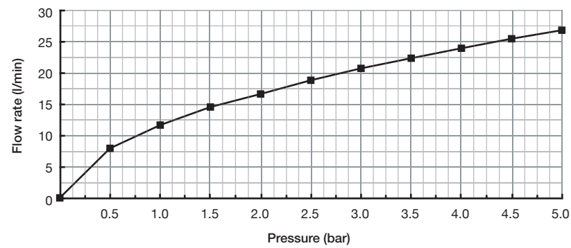
Thermostatic / pressure balance valve: R23-EM
